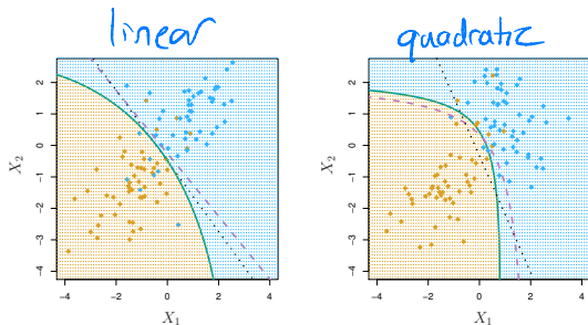
Figure 4.9 from ISL. Dashed purple curve is the Bayes classifier decision boundary. Solid green curve is QDA, dotted black line is LDA. Left: True boundary is linear. Right: True boundary is quadratic
